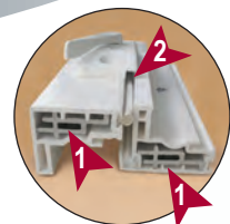
1) OPTIONAL metal reinforced, sash provides strength. Comes standard on windows over 48". 2) Interlocking sashes provide compression seal for maximum energy efficiency.
