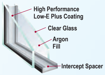
High-Performance Low-E Plus
