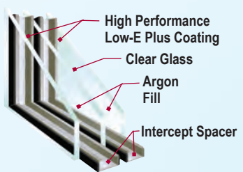
Ultra Triple Glazed
