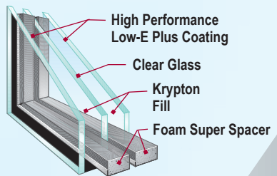
Ultimate Triple Glazed
